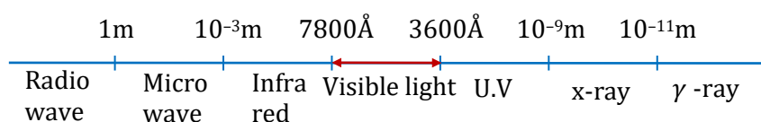
Electromagnetic spectrum
